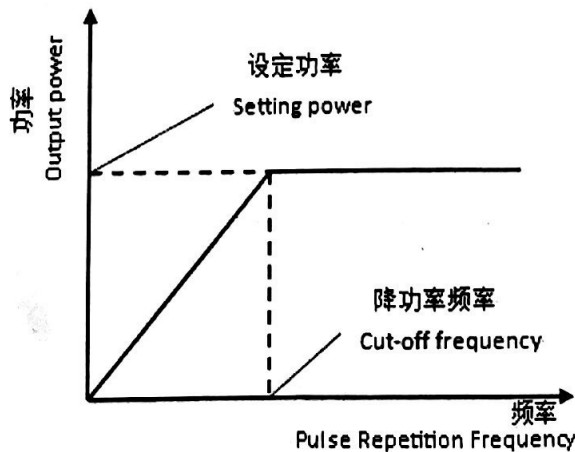
Fig.3 Relationship between Cut-off Frequency & Output power
