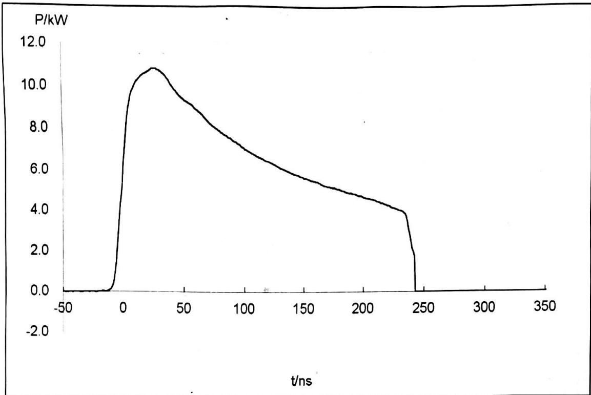
Fig.1 Waveform at 250ns/37kHz
