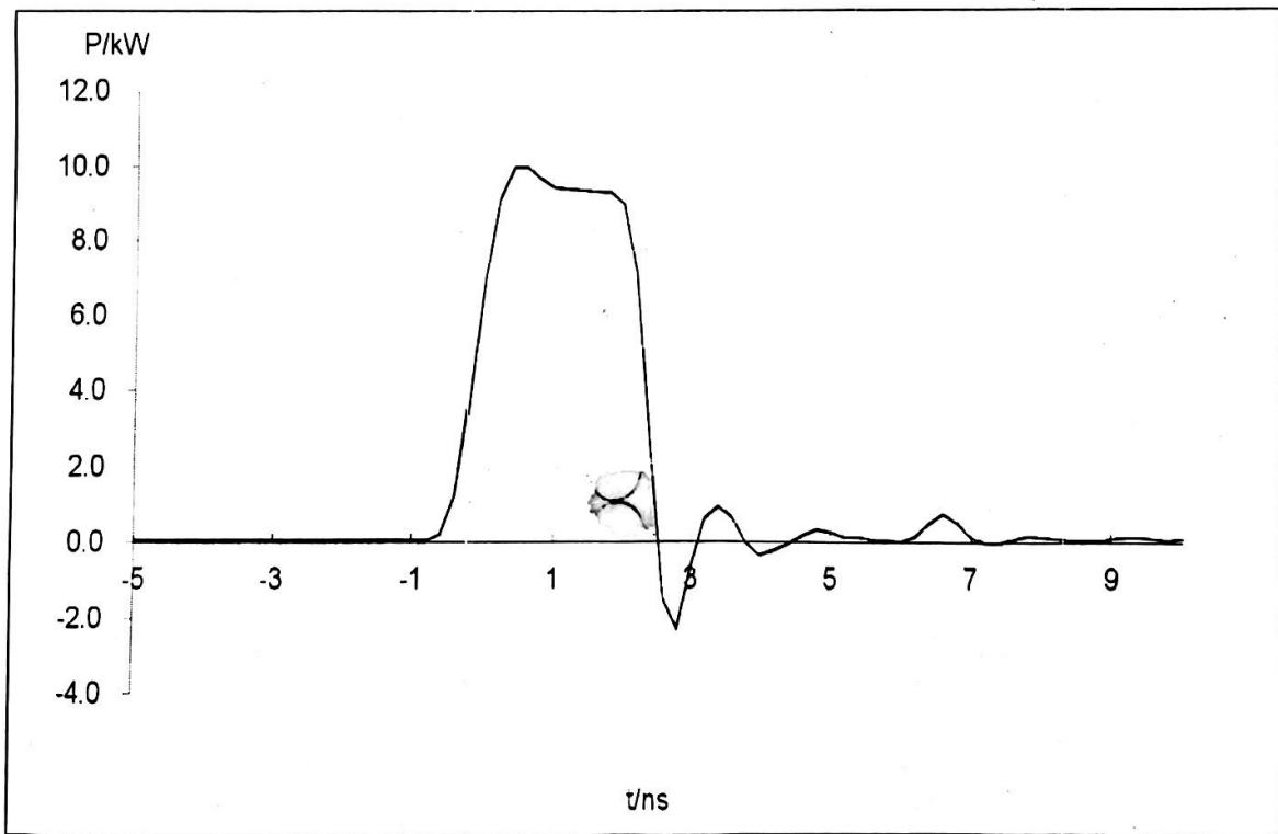
Fig.2 Waveform at 2ns/1950kHz
