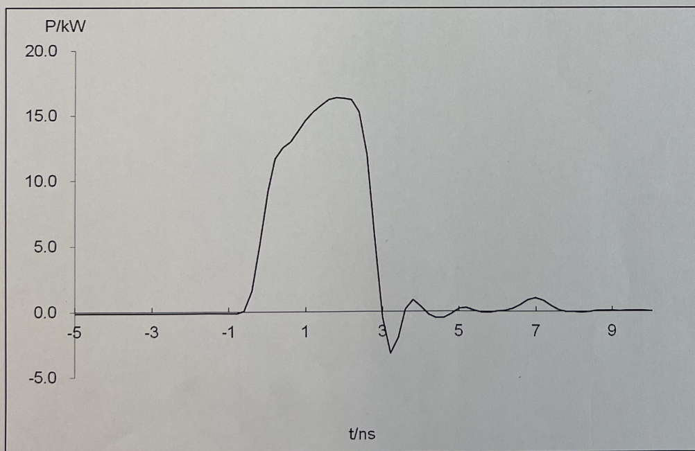
Fig.2 Waveform at 2ns/2600kHz
