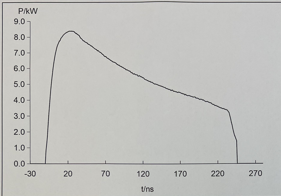
Fig.1 Waveform at 250ns/56kHz
